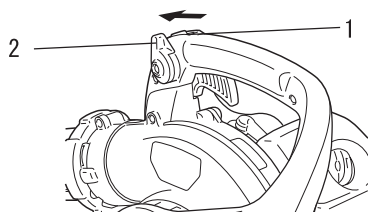
1. Stop switch 2. Throttle position lever
