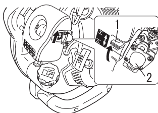
1. Choke 2. Purge bulb
